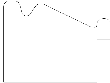
1587 Backband 1.417" x 1.875"
