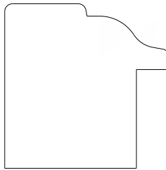
1041 Backband 1.250" x 1.250"
