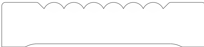
1516 Casing 0.750" x 3.500"
