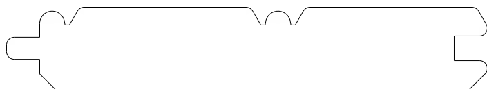
5200 Planking 0.625" x 3.625"
