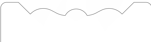
1823 Rosette 0.875" x 3.250"
