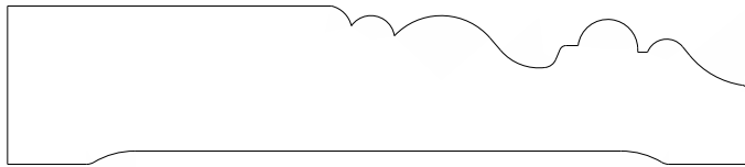
1568 Casing 0.750" x 3.500"
