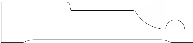
1540 Casing 0.750" x 3.500"
