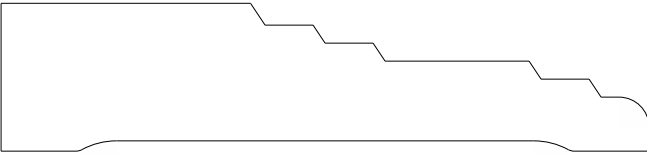
I534 Casing 0.750" x 3.375"
