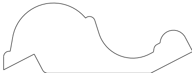
8550 Panel mold 0.750" x 2.000"
