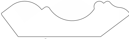
2525 Crown 0.750" x 2.250"
