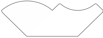
2531 Crown 0.625" x 1.750"
