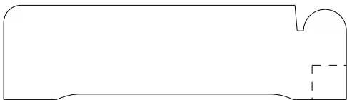
4225 Chair rail 0.687" x 2.500"
