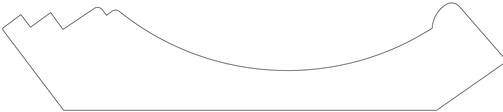
2563 Crown 1.090" x 5.315"
