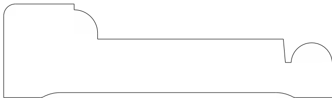
I207 Casing 1.000" x 3.500"
