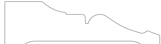
1522 Casing 0.875" x 3.187"
