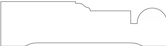
I244 Casing 0.750" x 2.750"
