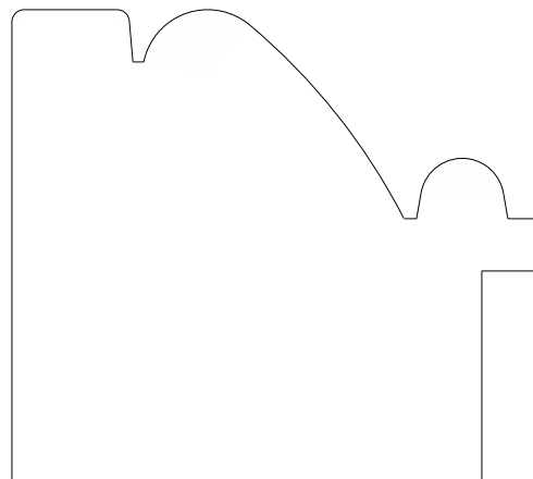
1690 Backband 2.250" x 2.500"
