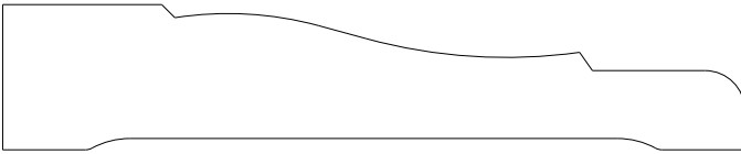
1004 Casing 0.687" x 3.500"
