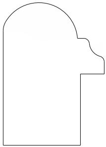
1511 Backband 1.500" x 1.062"
