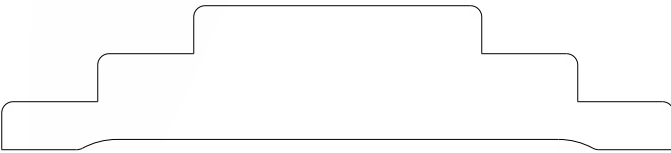
1710 Casing 0.750" x 3.500"
