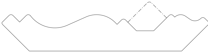
2045 Crown 0.750" x 4.250"
