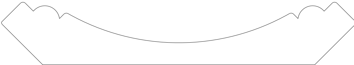
2566 Crown 1.062" x 6.000"
