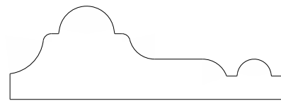
4076 Chair rail 0.687" x 2.000"
