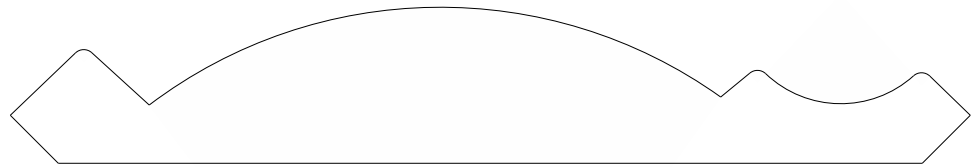
2554 Crown 0.812" x 5.000"
