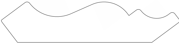
2030 Crown 0.750" x 3.250"
