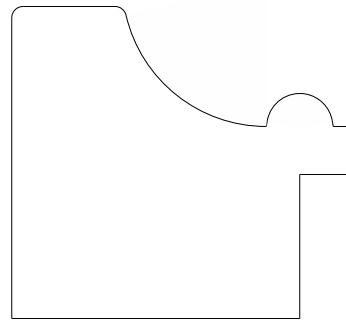
1580 Backband 1.625" x 1.750"
