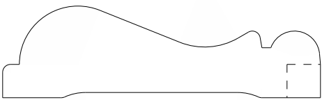
4055 Chair rail 0.687" x 2.375"
