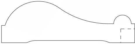
4037 Chair rail 0.750" x 2.375"
