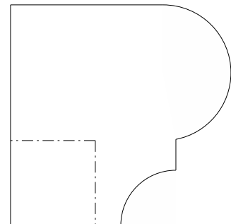
4585 Nosing 1.625" x 1.625"
