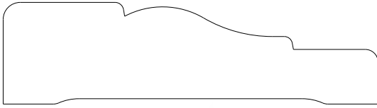
IO16 Casing 0.750" x 2.750"
