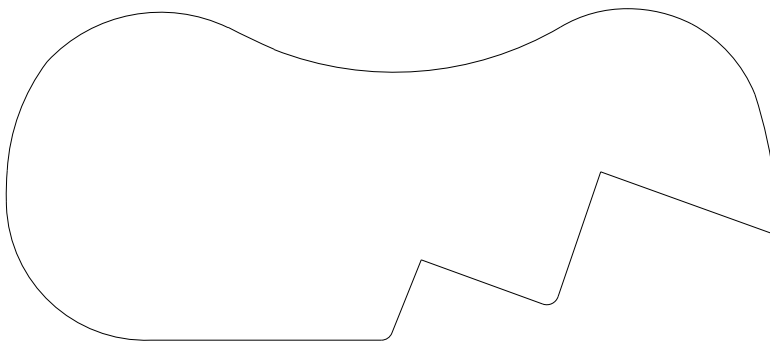
7768 Rail 1.726" x 4.000"
