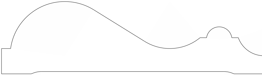
1057 Casing 1.250" x 4.500"
