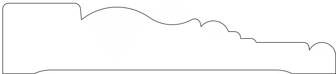
1059 Casing 0.750" x 3.500"
