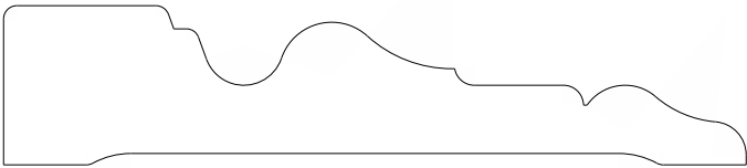
IO42 Casing 0.750" x 3.500"
