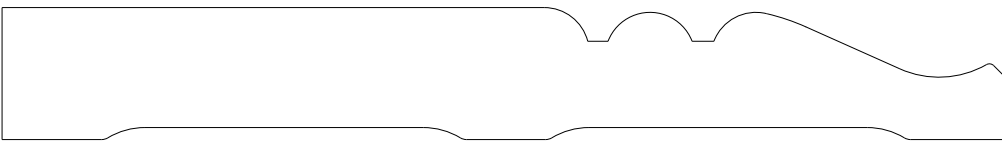
3538 Base 0.687" x 5.250"
