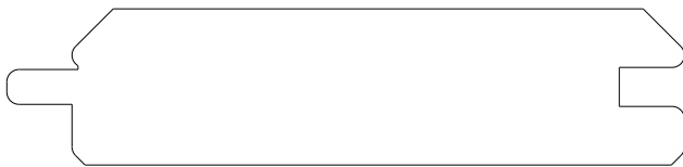
5300 Planking 0.750" x 3.250" , 4.250" , 5.250"
