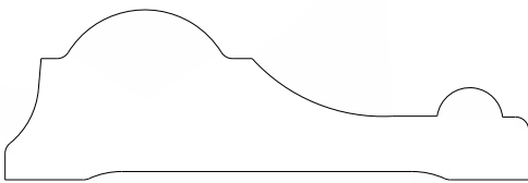
4523 Chair rail 0.812" x 2.500"
