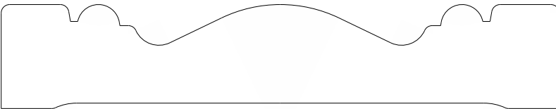
I549 Casing 0.750" x 4.125"
