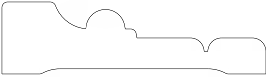
1525 Casing 0.750" x 2.750"
