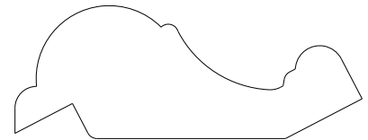
8549 Panel mold 0.750" x 2.000"
