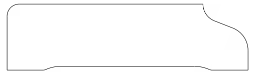
4065 Chair rail 0.687" x 2.500"
