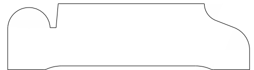
4240 Chair rail 0.687" x 2.500"
