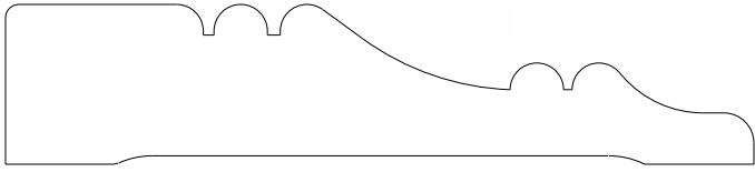
1056 Casing 0.750" x 3.500"
