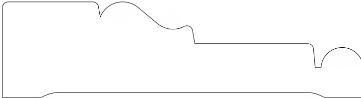
I247 Casing 1.000" x 3.750"
