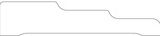
I536 Casing 0.750" x 3.500"
