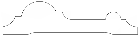
4520 Chair rail 0.687" x 2.750"
