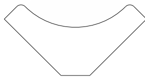
2511 Cove 0.750" x 1.500"
