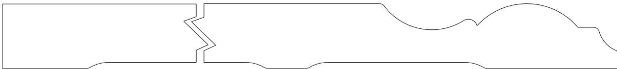
3524 Base 0.687" x 7.500"
