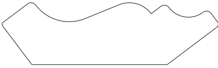
2020 Crown 0.625" x 2.250"
