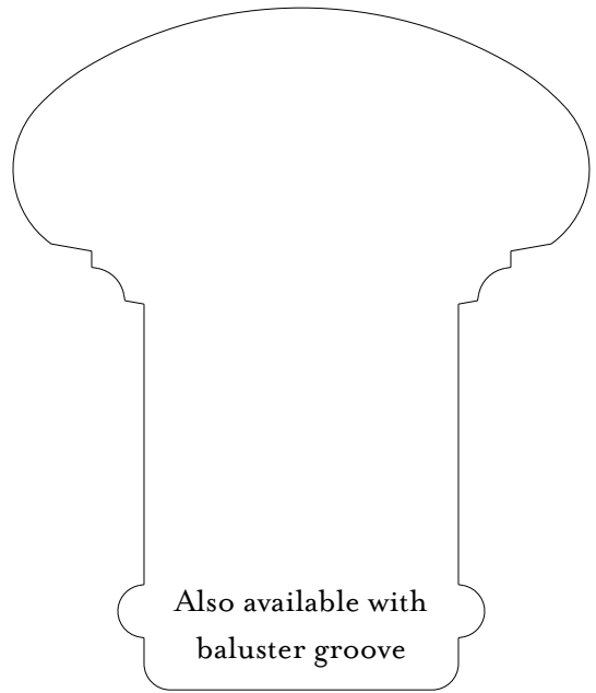
4551 Handrail 3.250" x 2.750"
