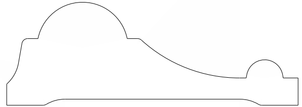
4522 Chair rail 1.062" x 3.000"
