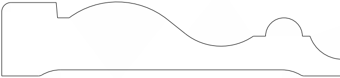
IO31 Casing 0.750" x 3.500"
