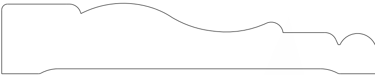
IO67 Casing 0.750" x 4.000"
